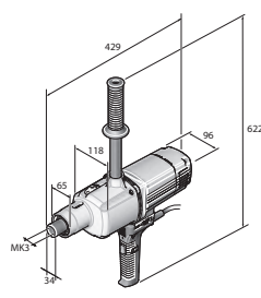
BOZ 32-4 M
