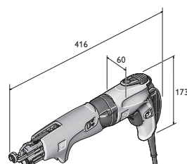
SCT 5-40 M
