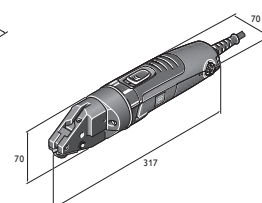
BSS 2.0 E
