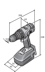
ABS 18 Q
